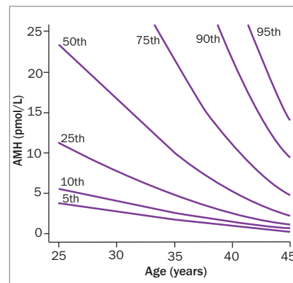
Figure 2. Predicted anti-Müllerian hormone (AMH) level versus age, showing the 5th, 10th, 25th, 50th, 75th, 90th and 95th percentiles of the distribution. The nomogram is based on a quadratic model of log(AMH) on age.
